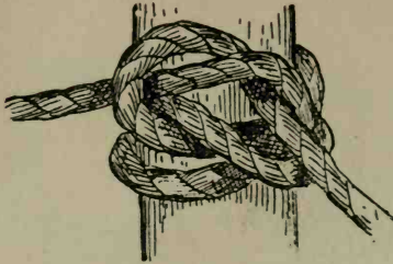
FIG. 37.—Gunner's knot.
